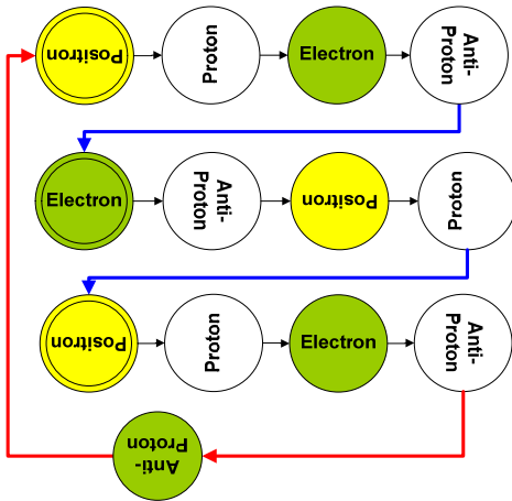
Figure 20. Pion Plus diagram.
