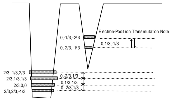
Figure 16. Electron-positron transmutation note.
